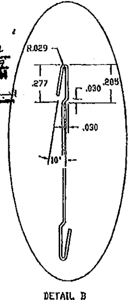
DETAIL B
