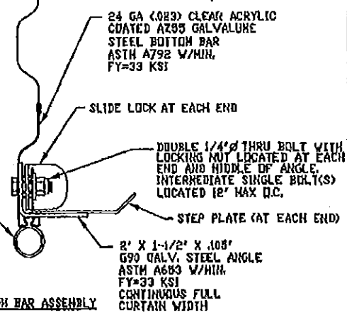
BOTTOM BAR ASSEMBLY
